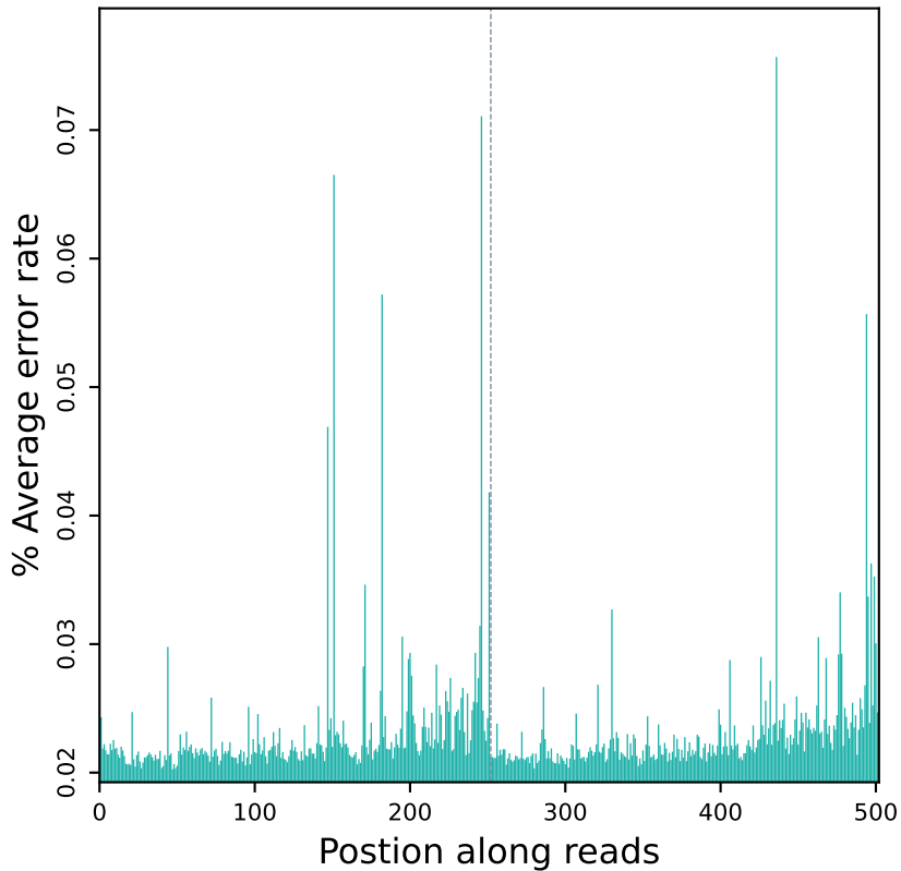
Error rate distribution along reads (R10221)
